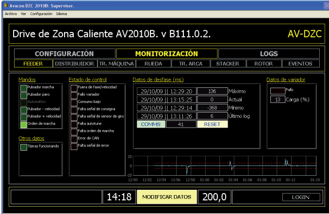
Drive Supervisor.
